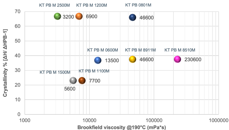
Illustration of Koattro Polybutene-1 portfolio as a function of Brookfield viscosity @190°C (mPa*s) and crystallinity (%)
